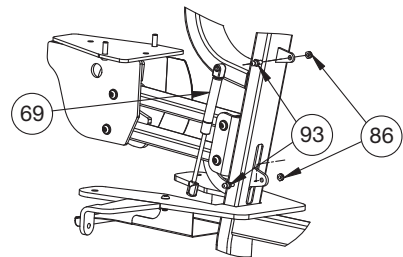
SEAT GAS SPRING ASSEMBLY DETAIL
