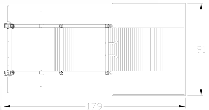
XXL-2960 / XXL-912 L 179" W 91" H 100"
